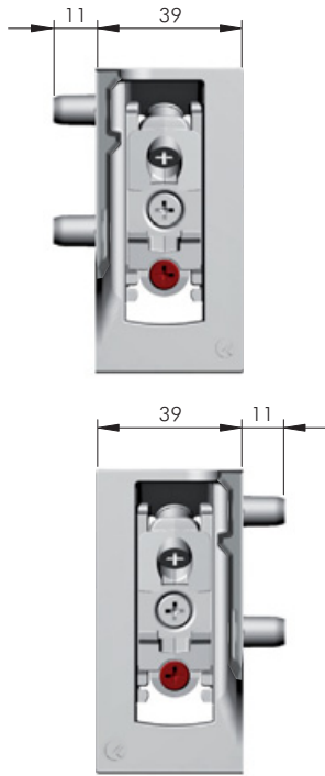
DRILLING PLAN WITHOUT BACK PANEL
